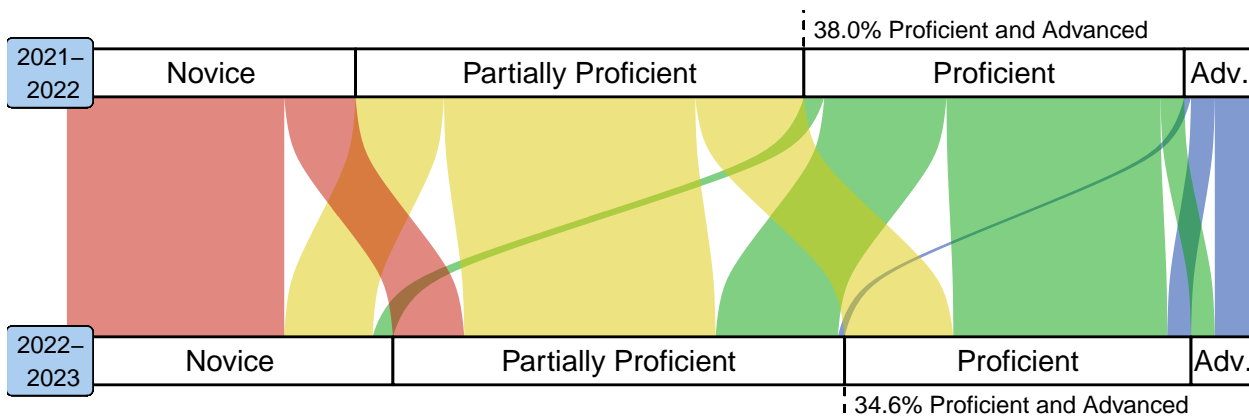
Figure 1: NDSA Mathematics proficiency transition for students of Dickinson State University first year teachers
